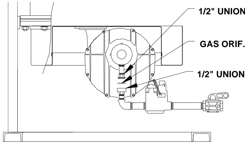
Fig 1. REPLACE ORIFICE
