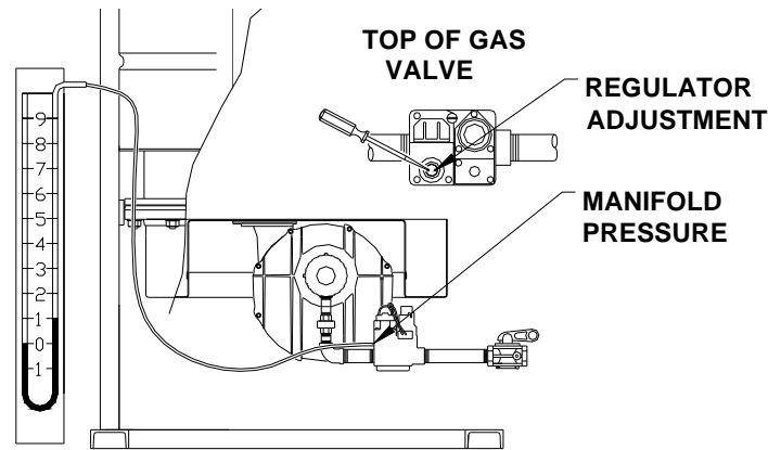
Fig 2. ADJUST REGULATOR
