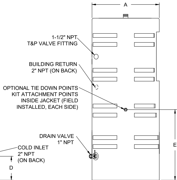
LEFT VIEW
