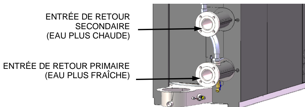
Figure 2-8 : Double retour
