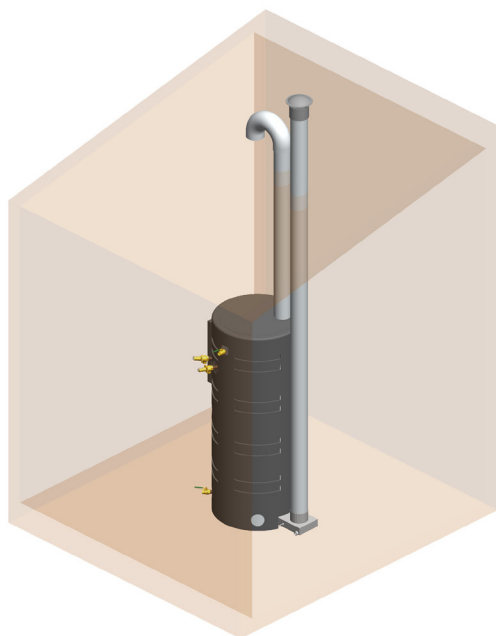
Sealed combustion with roof terminations
